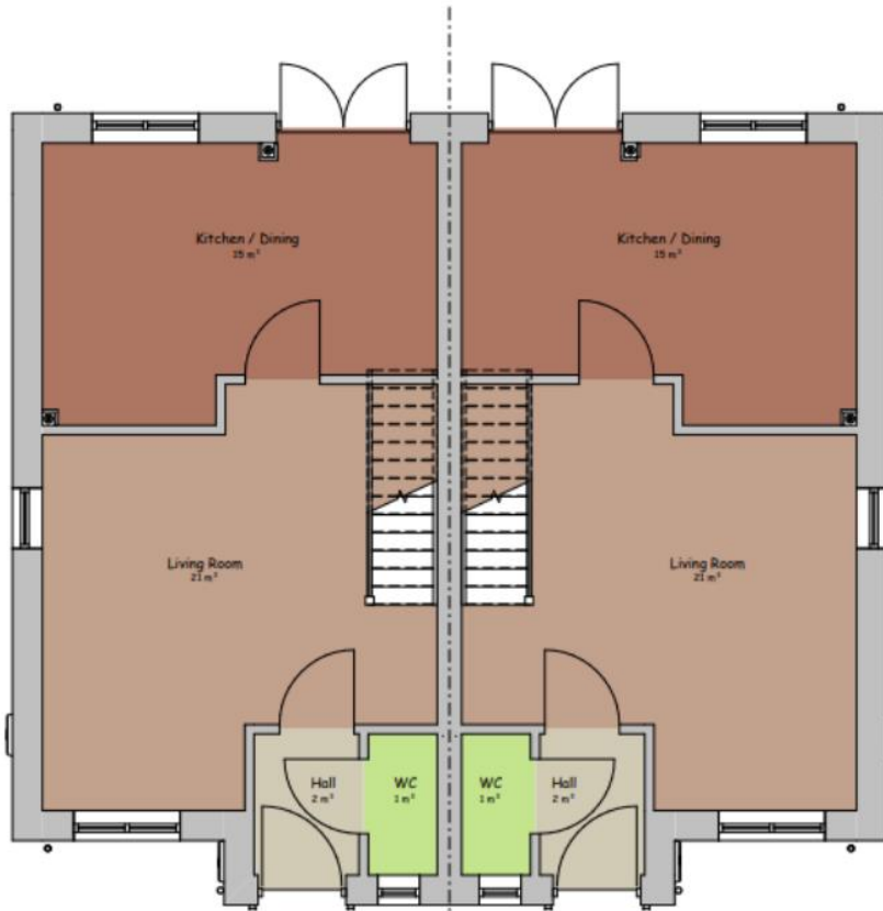
Proposed Ground Floor - Accommodation Schedules 1 : 50
