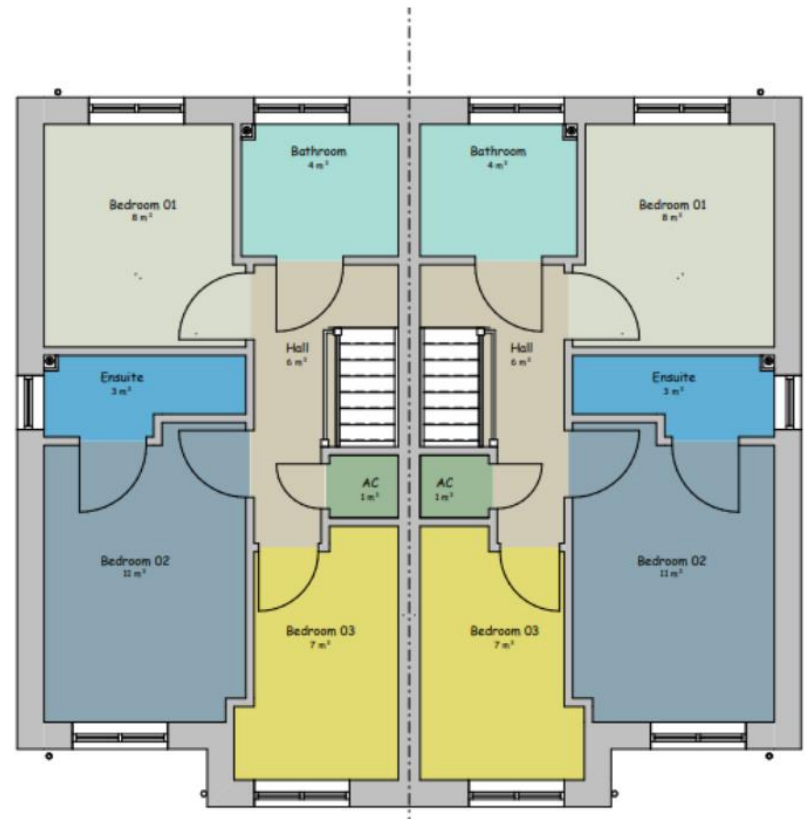
Proposed First Floor - Accommodation Schedules 1 : 50
